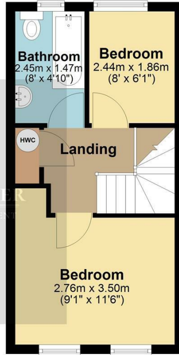
First Floor Approx. 25.2 sq. metres (271.0 sq. feet)
